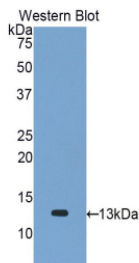
Figure. Western Blot; Sample: Recombinant MCP1, Rabbit.
