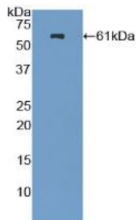
Figure. Western Blot; Sample: Recombinant NES, Mouse.
