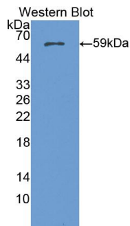
Figure. Western Blot; Sample: Recombinant NUP188, Human.
