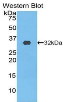
Figure. Western Blot; Sample: Recombinant PIK3C2b, Rat.
