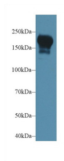
Western Blot; Sample: Rat Serum; Primary Ab: 1µg/ml Rabbit Anti-Rat PIK3C2b Antibody Second Ab: 0.2µg/mL HRP-Linked Caprine Anti-Rabbit IgG Polyclonal Antibody (Catalog: SAA544Rb19)
