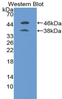
Figure. Western Blot; Sample: Recombinant PLGF, Mouse.
