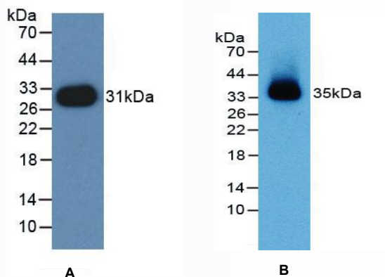
Figure 1. Western Blot
