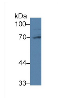
Western Blot; Sample: Rat Liver lysate; Primary Ab: 2 \mu g/ml Rabbit Anti-Human PABPC1L Antibody Second Ab: 0.2 \mu g/mL HRP-Linked Caprine Anti-Rabbit IgG Polyclonal Antibody (Catalog: SAA544Rb19)
