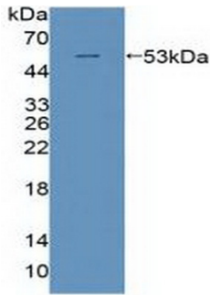
Figure. Western Blot; Sample: Recombinant POLd, Human.
