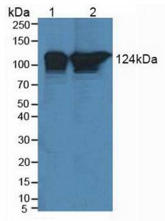
Figure. Western Blot; Sample: Lane1: Human Jurkat cells; Lane2: Human HeLa cells.
