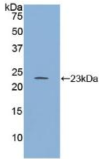
Figure. Western Blot; Sample: Recombinant RGS4, Human.
