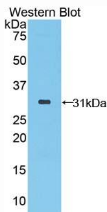
Used in Western Blot, Sample: Recombinant STAMPB, Human
