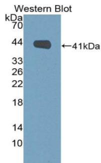
Figure. Western Blot; Sample: Recombinant SCGB3A1, Human.
