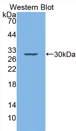
Used in Western Blot, Sample: Recombinant SEPN1, Human
