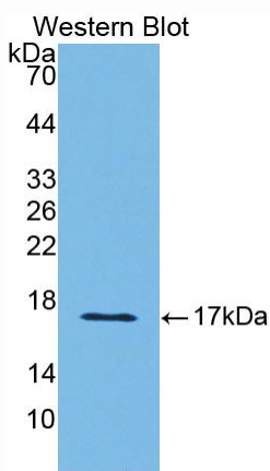
Used in Western Blot, Sample: Recombinant SEMA3A, Mouse
