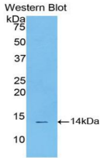
Figure. Western Blot; Sample: Recombinant STAT3, Bovine.
