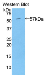
Figure. Western Blot; Sample: Recombinant TGM1, Human.
