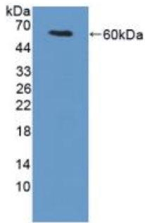
Figure. Western Blot; Sample: Recombinant TGM1, Mouse.
