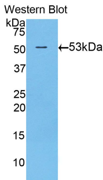
Used in Western Blot, Sample: Recombinant TGM1, Rat
