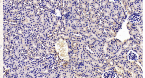
DAB staining on IHC-P; Sample: Mouse Kidney Tissue; Primary Ab: 10ug/ml Rabbit Anti-Human TWSG1 Antibody Second Ab: 2µg/mL HRP-Linked Caprine Anti-Rabbit IgG Polyclonal Antibody (Catalog: SAA544Rb19)
