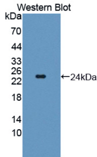
Figure. Western Blot; Sample: Recombinant TWSG1, Human.
