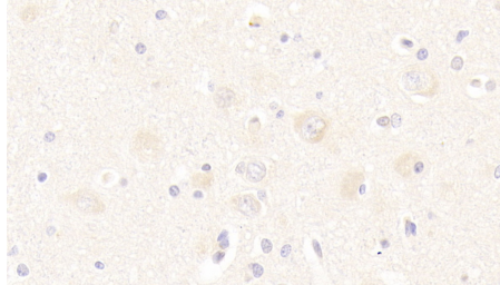
DAB staining on IHC-P; Samples: Human Cerebrum Tissue; Primary Ab: 20?g/ml Rabbit Anti-Human TWSG1 Antibody Second Ab: 2µg/mL HRP-Linked Caprine Anti-Rabbit IgG Polyclonal Antibody (Catalog: SAA544Rb19)
