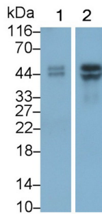
Western Blot; Sample: Lane1: Porcine Bladder lysate; Lane2: Rat Bladder lysate Primary Ab: 0.1µg/ml Rabbit Anti-Human UPK3A Antibody Second Ab: 0.2µg/mL HRP-Linked Caprine Anti-Rabbit IgG Polyclonal Antibody (Catalog: SAA544Rb19)
