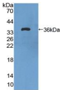
Figure. Western Blot; Sample: Recombinant VEGFR1, Rat.
