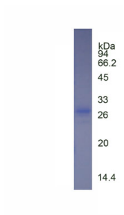
Figure. SDS-PAGE
