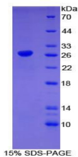
Figure. SDS-PAGE
