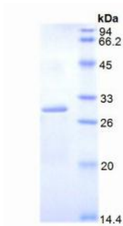
Figure. SDS-PAGE
