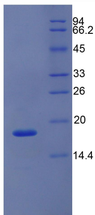
Figure 1. SDS-PAGE
