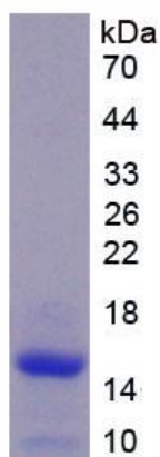
Figure 1. SDS-PAGE
