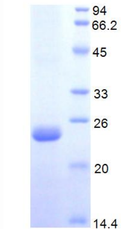
Figure 1. SDS-PAGE
