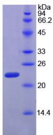
Figure 1. SDS-PAGE
