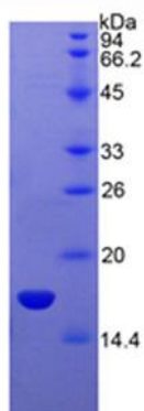
Figure 2. SDS-PAGE
