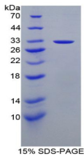
Figure. SDS-PAGE
