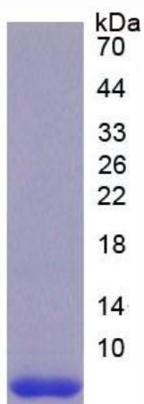
Figure 2. SDS-PAGE
