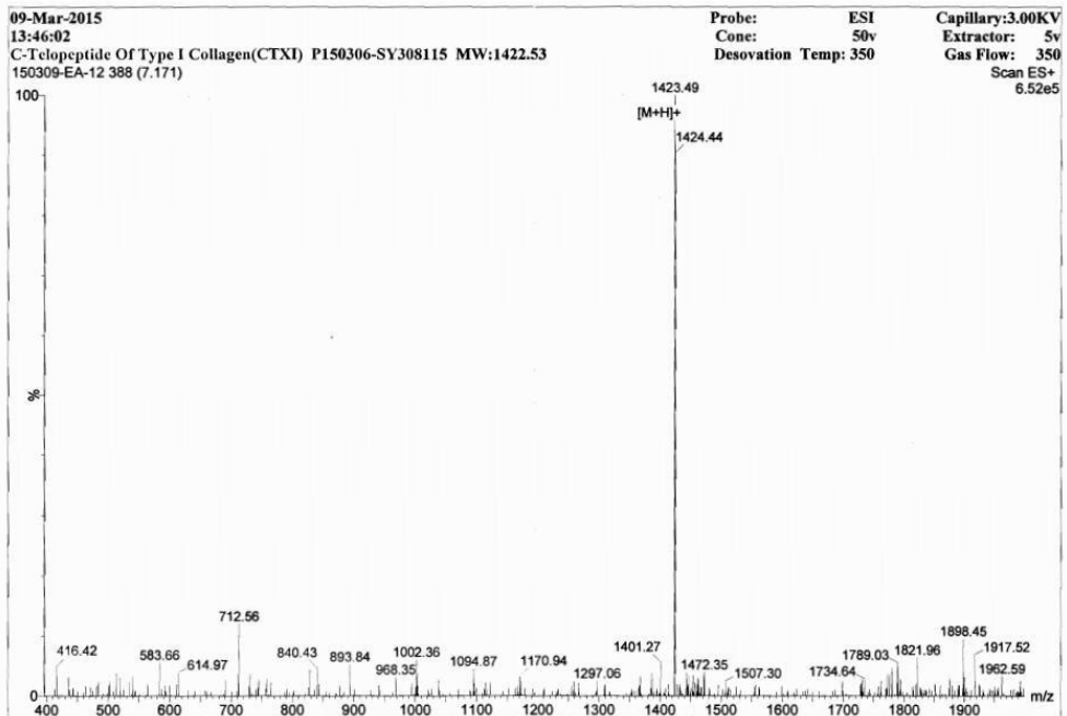
Figure 2. MASS Spectrometry
