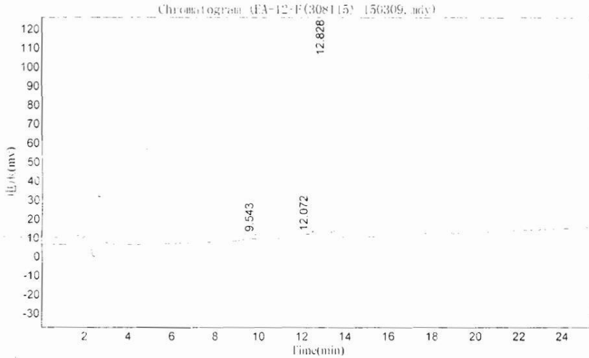
Figure 1. HPLC
